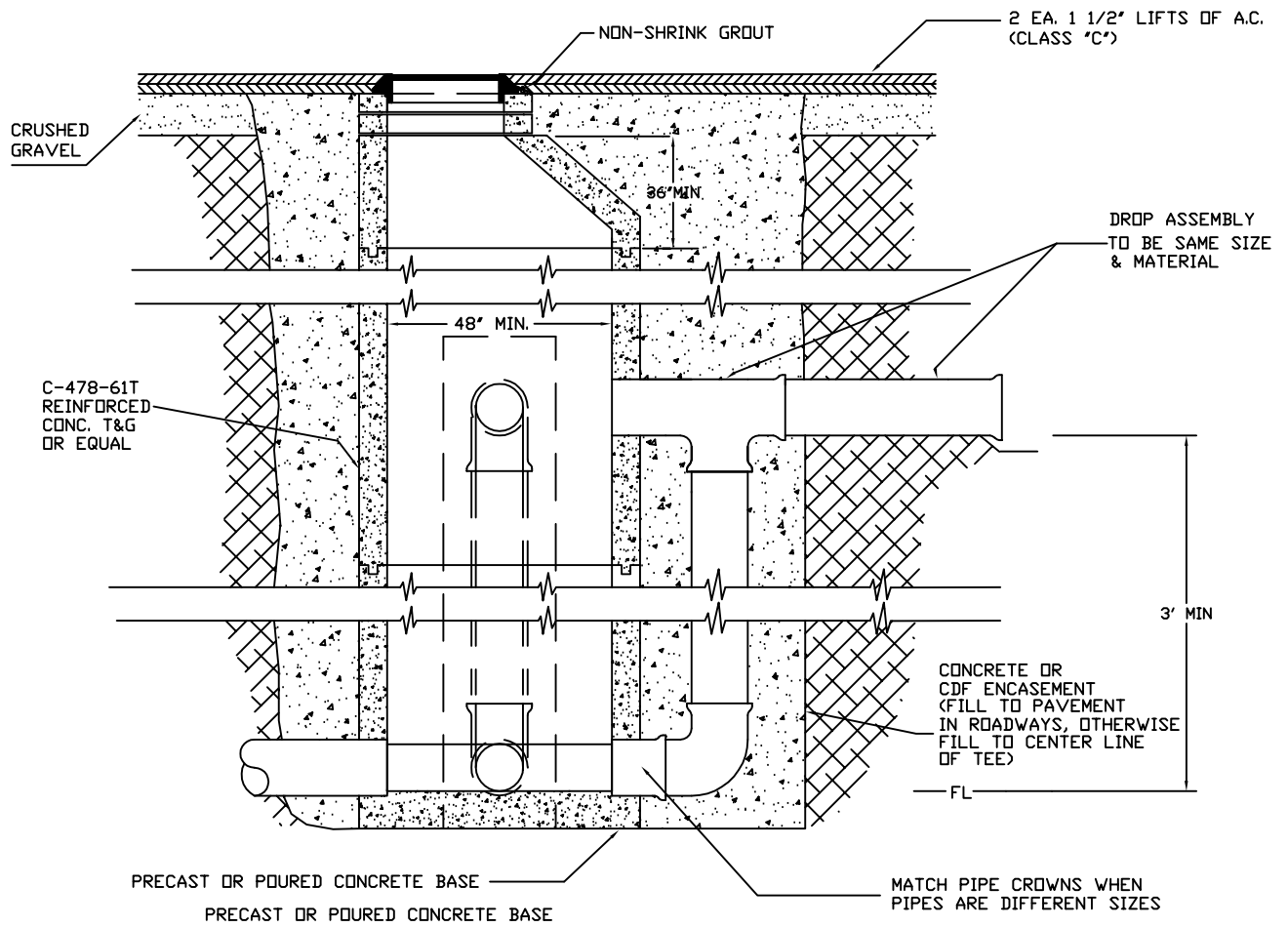
TYPICAL DROP MANHOLE
